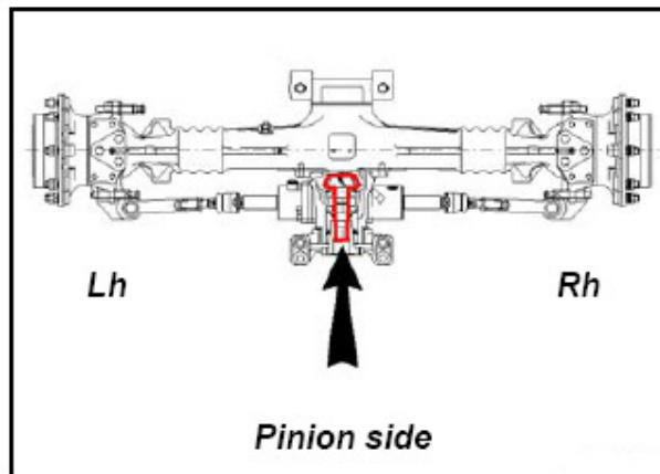
Figure 2 – Lh/Rh side on axles with pinion
